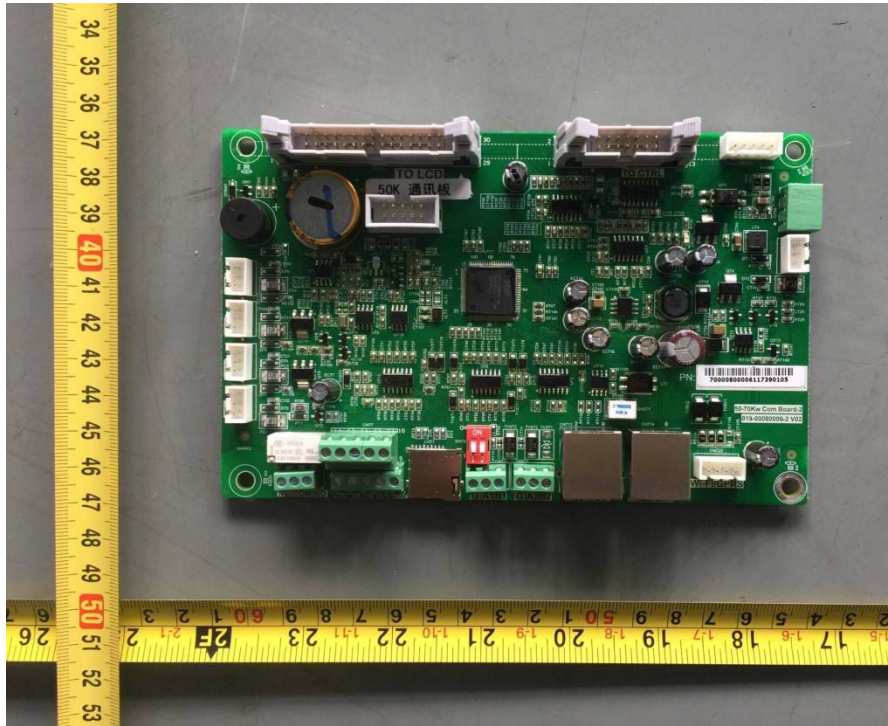
Components side of communication board view
