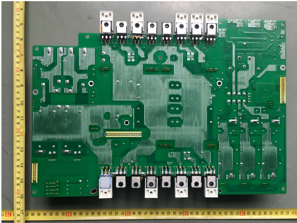
Trace side of main board view
