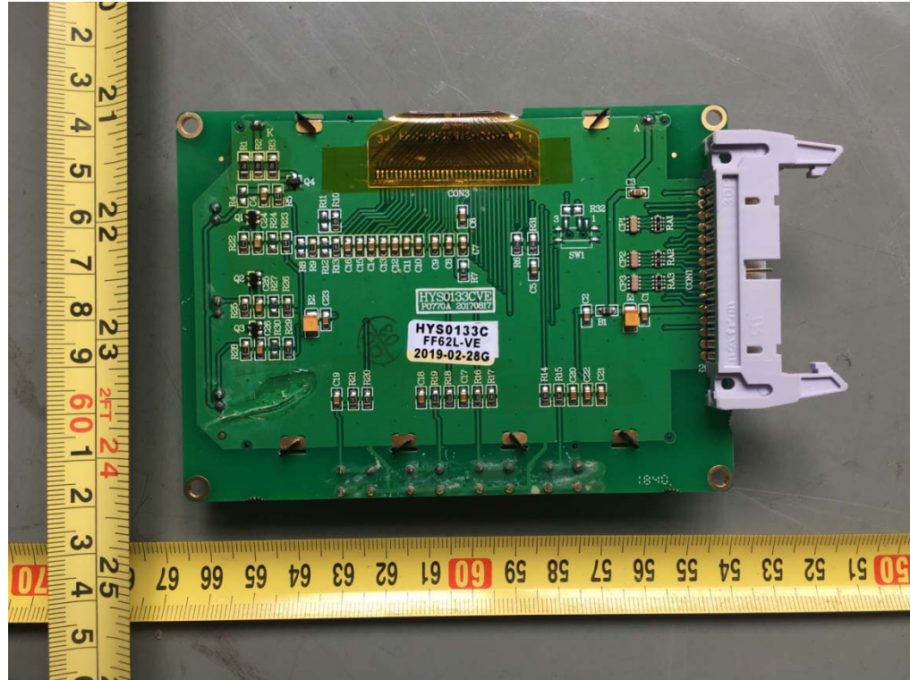
Trace side of LCD view
