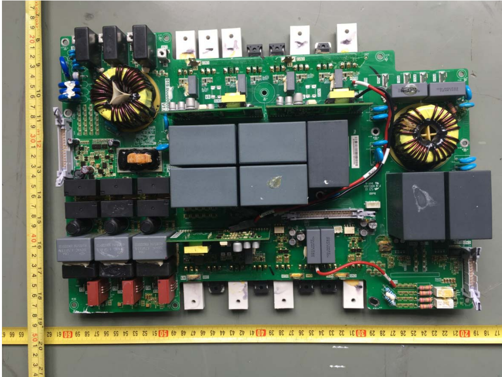
Component side of main board view
